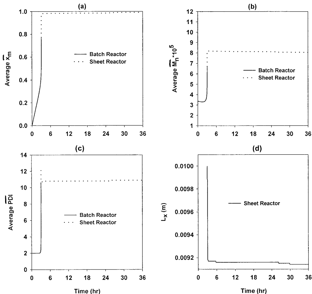
Figure 11 \bar{x}_m , \bar{M}_n , \overline{PDI} and L_x as a function of t in the two reactors. L_{,ini} = 0.01 m. All other decision variables are at their reference values.
