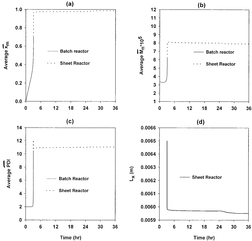
Figure 3 Section-average values of \bar{x}_m , \bar{M}_n , and \overline{PDI} , and half the sheet thickness, L_x , as a function of time, t , for the reference conditions. Solid lines represent the batch reactor while dotted lines represent the sheet reactor.
