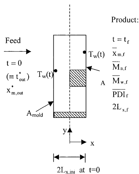
(b) Mold (Sheet Reactor), with a computational shell having an initial volume of V_{out}^* (= AL_{x,ini})
