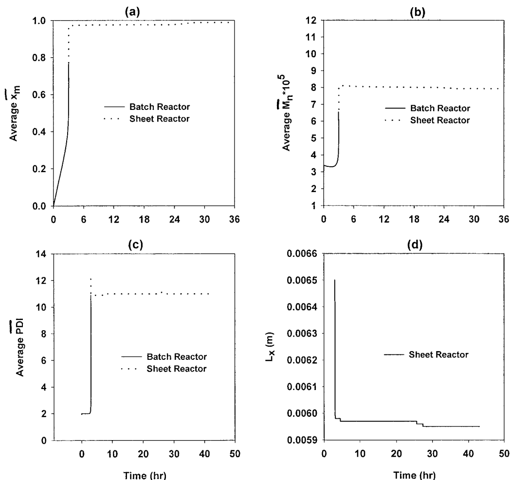
Figure 13 \bar{x}_m , \bar{M}_n , \bar{PDI} and L_x as a function of t in the two reactors. T_{w,\max} = 90^\circ\text{C} during 24\text{ h} \leq t \leq 27\text{ h} in the sheet reactor. All other decision variables are at their reference values.
