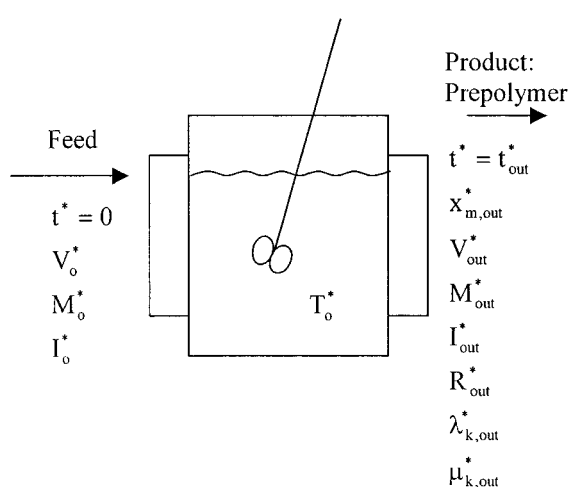
(a) Batch Reactor
